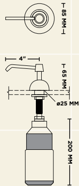
SCAL-128-4 Deck Mounted Soap Dispenser (4")
