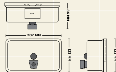
■ SCAL-124 Horizontal Wall Soap Dispenser (40oz)
