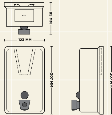
■ SCAL-126 Vertical Wall Soap Dispenser (40oz)
