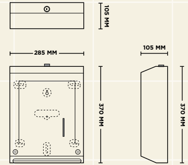
SCAL-162 Wall Mounted C-Fold Tissue Paper Dispenser
