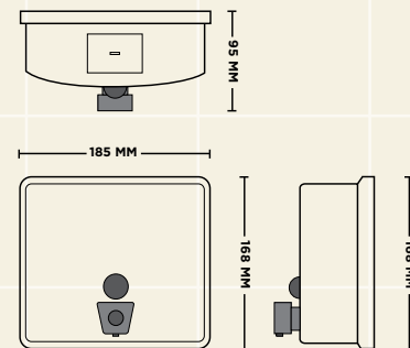
■ SCAL-124 Horizontal Wall Soap Dispenser (40oz)
