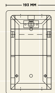
SCAL-188-R Recessed Dual Roll Toilet Tissue Dispenser
