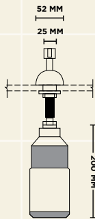
SCAL-128-4 Deck Mounted Soap Dispenser (4")
