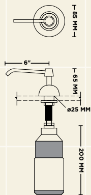
SCAL-128-6 Deck Mounted Soap Dispenser (6")
