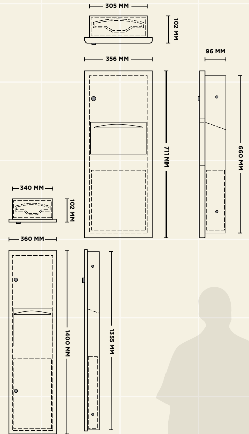
SCAL-162 Wall Mounted C-Fold Tissue Paper Dispenser
