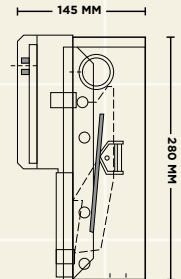
SCAL-188 Surface Mounted Dual Roll Toilet Tissue Dispenser
